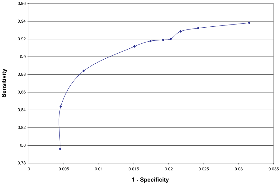
Fig. 1. ROC graph
