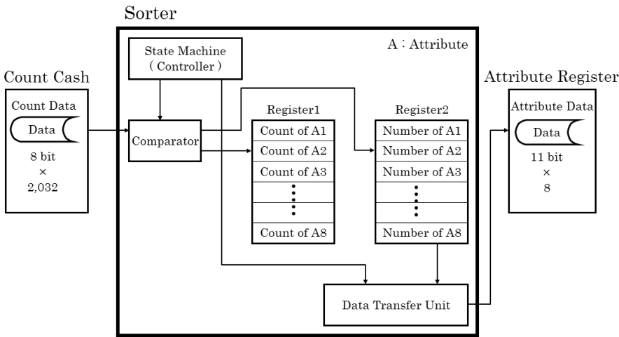
Fig. 8. Block diagram of Sorter
