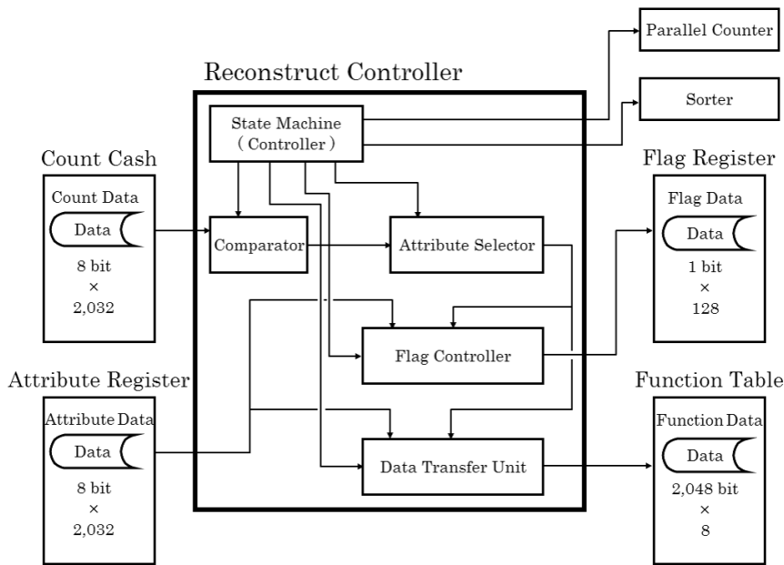
Fig. 9. Block diagram of Reconstruction Controller
