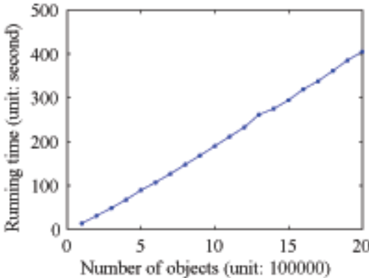
Fig. 1. Experiment results on KDD data sets
