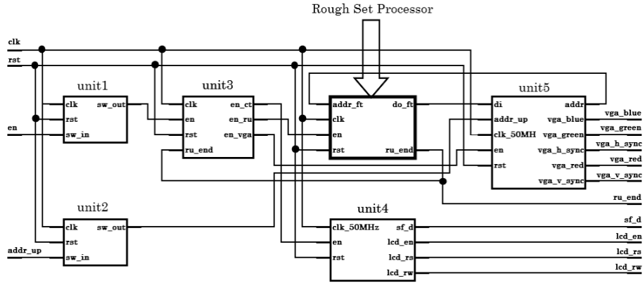
Fig. 10. Test Circuit
