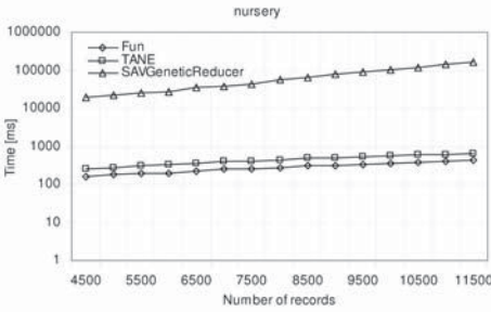
Fig. 1. nursery - logarithmic scale
