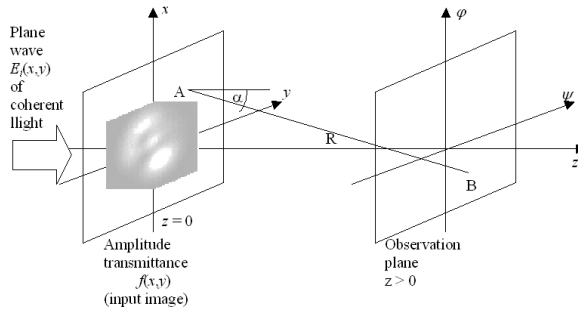
Fig. 1. The input plane with the transparent image f(x, y) and the observation plane with observation point B , are parallel to each other and perpendicular to the optical axis represented by the axis z of Cartesian coordinate system. Modified basing on [20].
