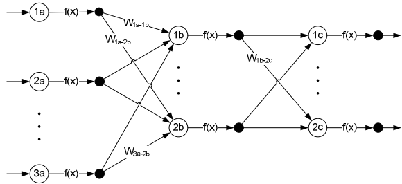
Fig. 1. A sample feed-forward neural network with 3 layers
