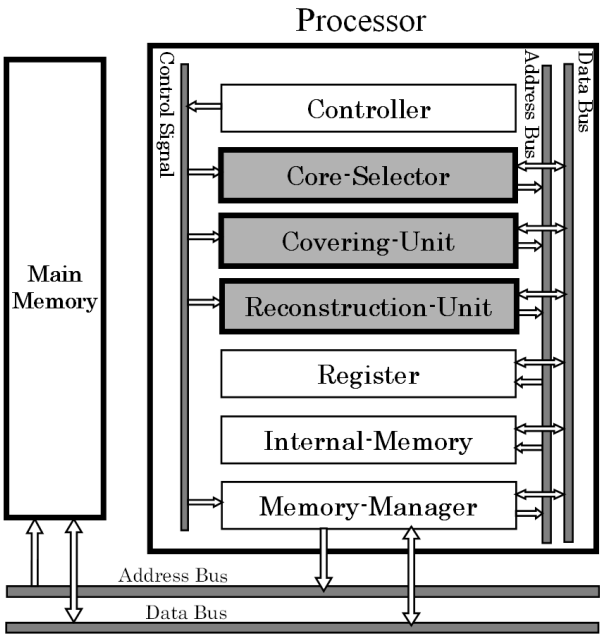
Fig. 2. Block diagram of proposed processor
